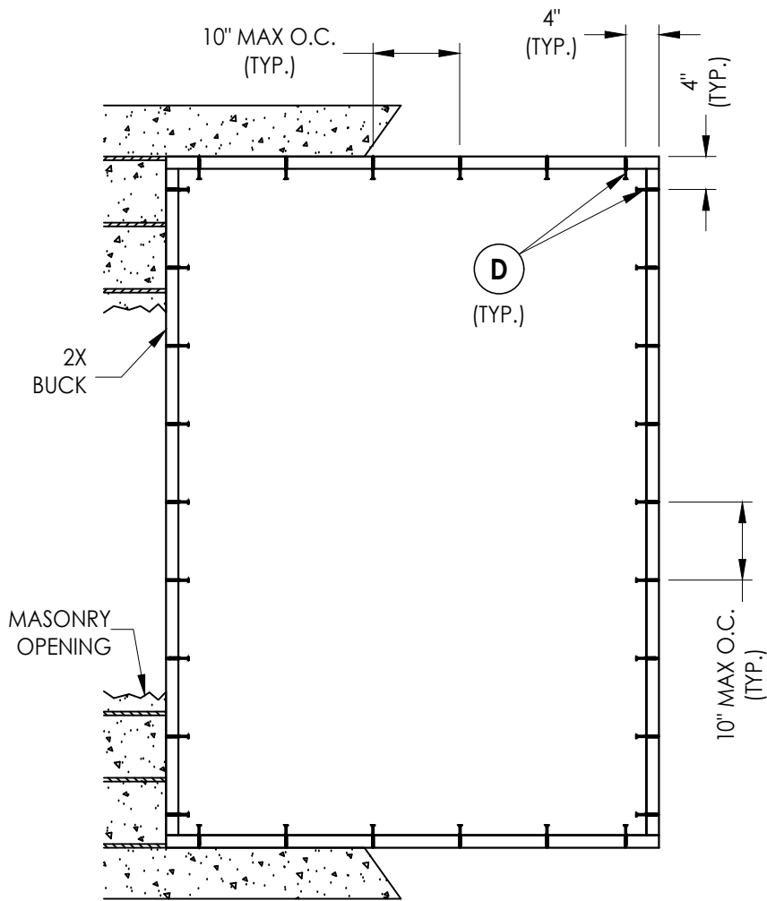
BUCK ANCHORING
