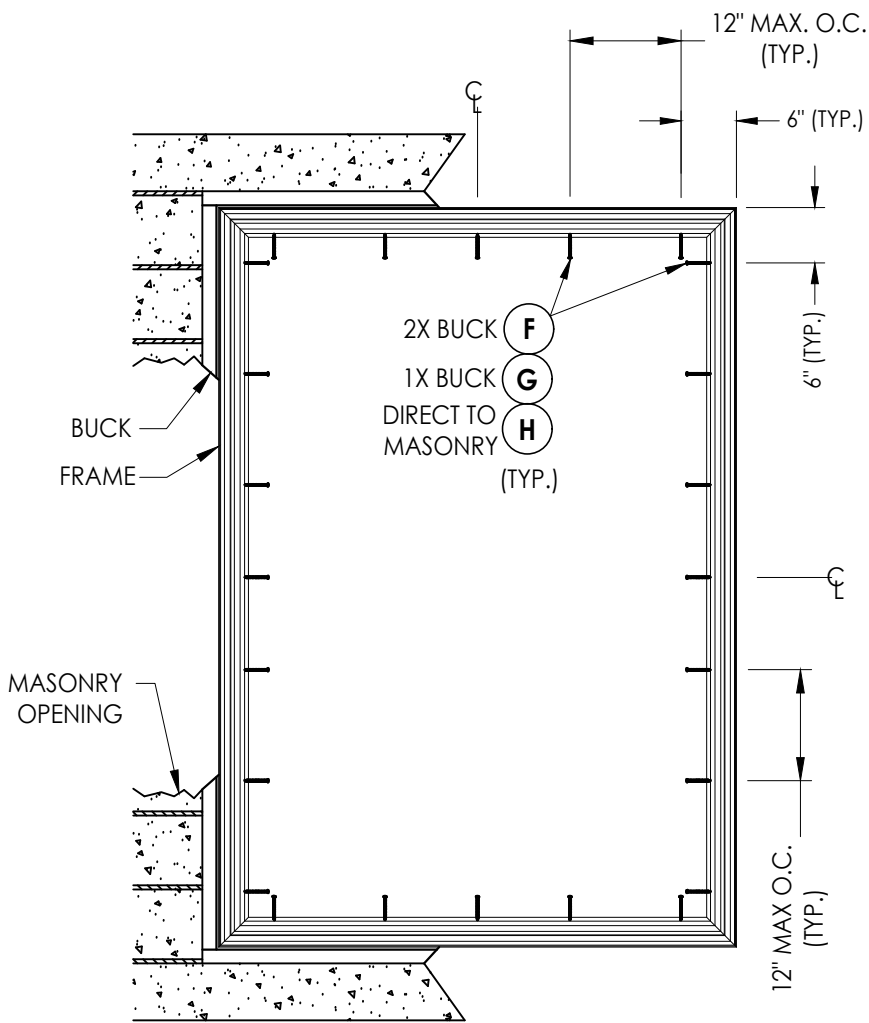
FRAME ANCHORING
